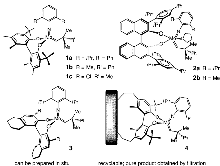
Scheme 1. Representative chiral Mo-based catalysts for olefin metathesis. TMS = Si-Me 3 , Tf = CF 3 SO 2 .
