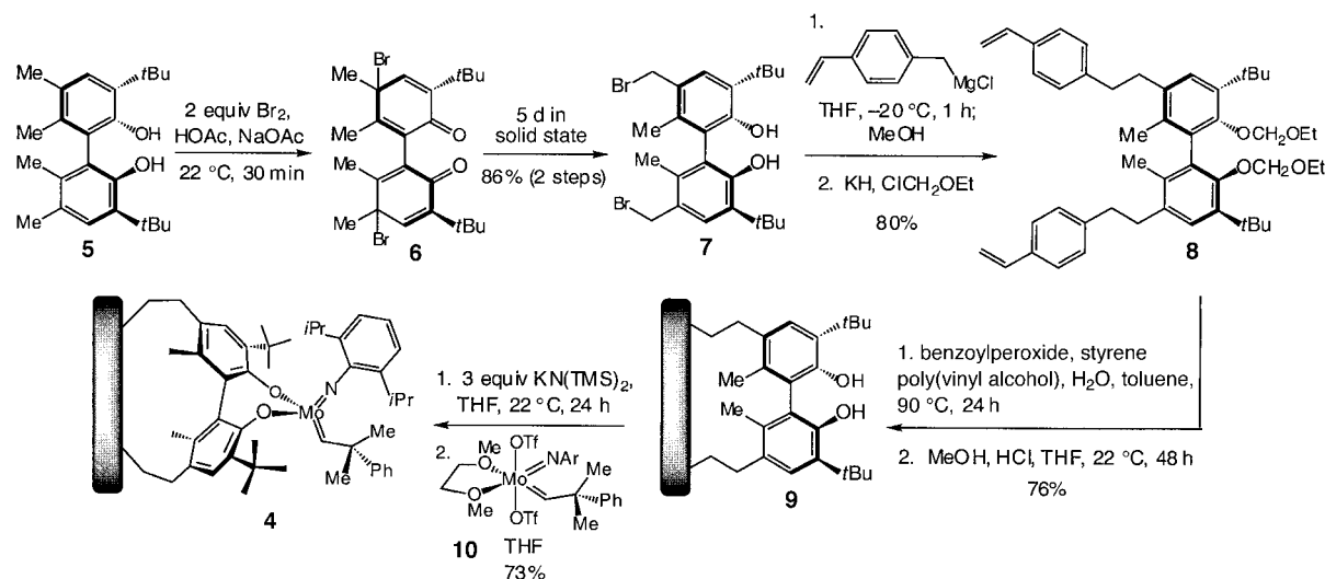
Scheme 2. Synthesis of supported chiral catalyst 4 .
